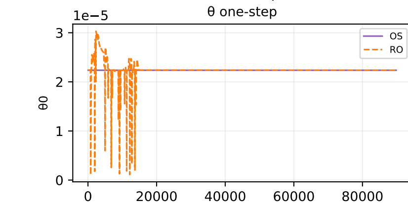
Oracle theta fit — sample 675
