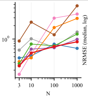
(b) Glycolysis/8-state
