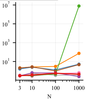
(c) Glycolysis/12-state
