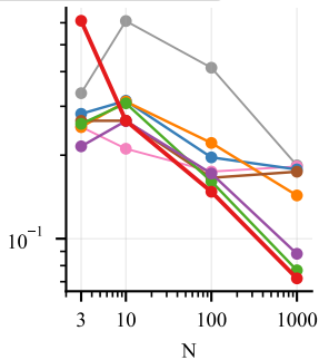
(c) Glycolysis/12-state
