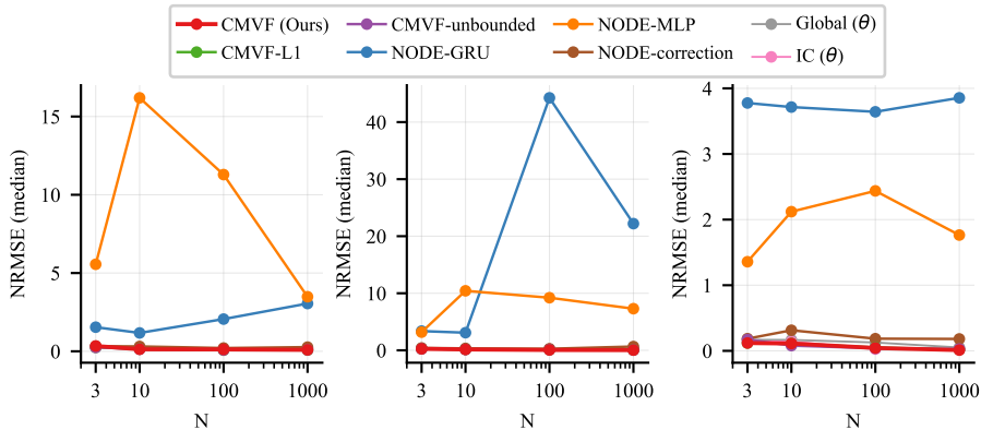
(a) MOF/6-state
