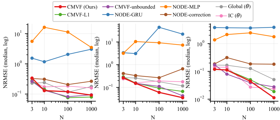
(a) MOF/6-state
