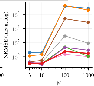
(c) MOF/12-state
