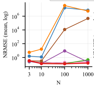
(a) MOF/6-state
