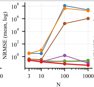
(b) MOF/8-state
