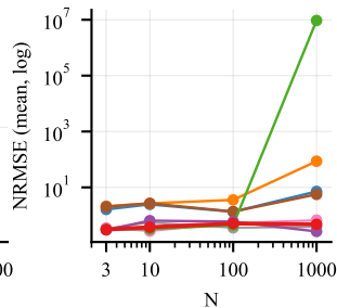
(f) Glycolysis/12-state
