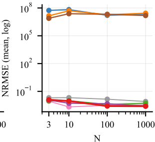
(i) Enzyme/6-state
