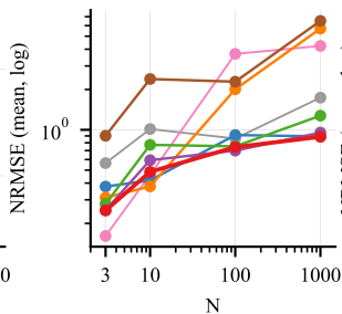
(e) Glycolysis/8-state
