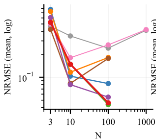
(g) Enzyme/2-state
