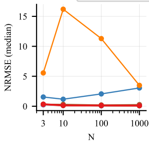
(a) MOF/6-state
