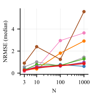
(e) Glycolysis/8-state
