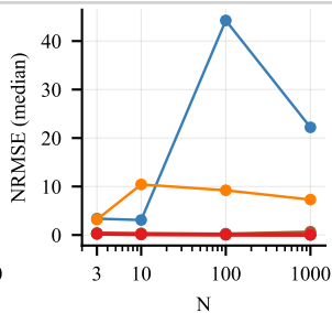
(b) MOF/8-state
