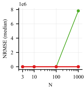
(f) Glycolysis/12-state
