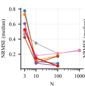
(g) Enzyme/2-state
