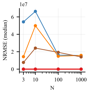
(i) Enzyme/6-state
