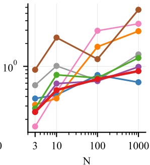
(b) Glycolysis/8-state
