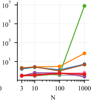
(c) Glycolysis/12-state
