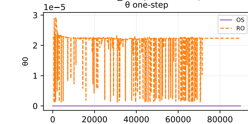
Oracle theta fit — ivtt_analytic — sample 141
