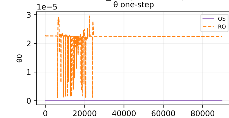
Oracle theta fit — ivtt_analytic — sample 146
