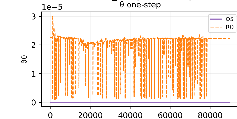
Oracle theta fit — ivtt_analytic — sample 245
