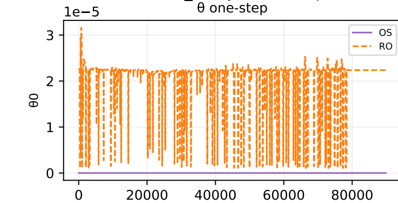
Oracle theta fit — ivtt_analytic — sample 261
