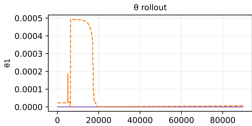
Oracle theta fit — ivtt_analytic — sample 359
