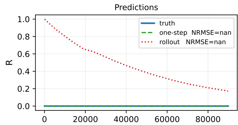
Oracle theta fit — ivtt_analytic — sample 359
