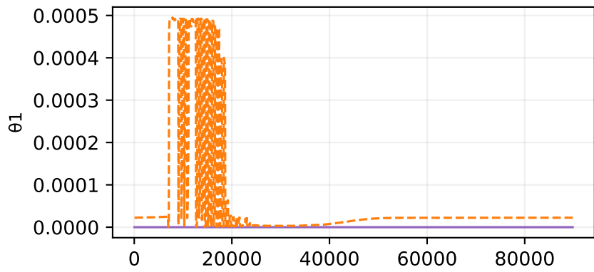
\theta rollout
