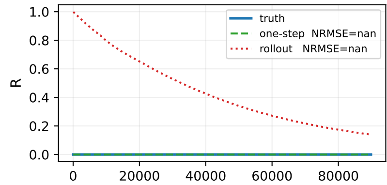
Predictions
