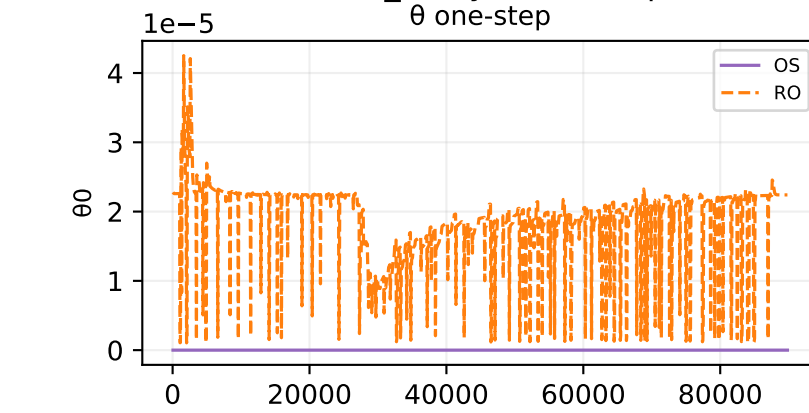
Oracle theta fit — ivtt_analytic — sample 497
