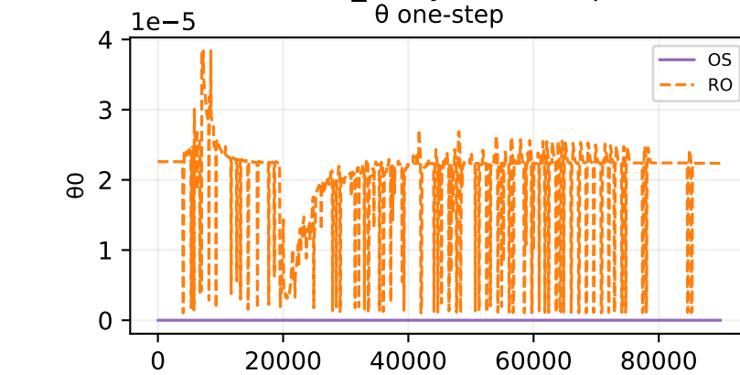
Oracle theta fit — ivtt_analytic — sample 544
