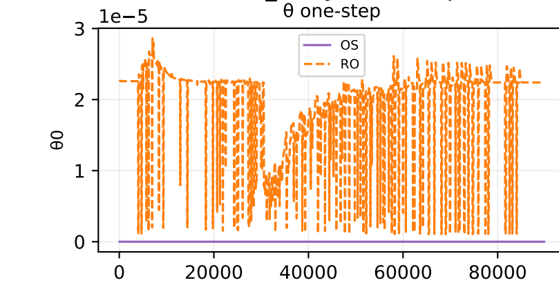
Oracle theta fit — ivtt_analytic — sample 554
