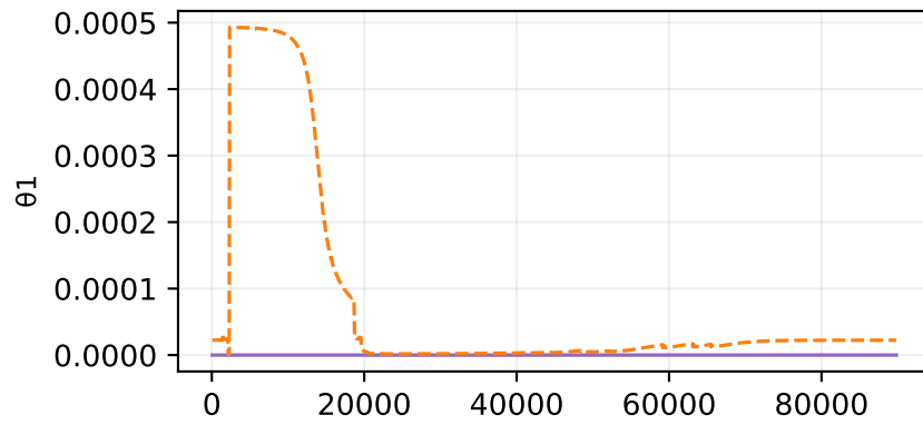
\theta rollout
