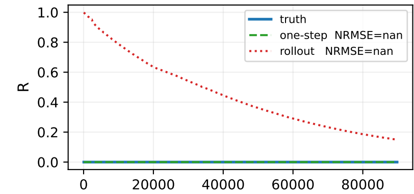
Predictions
