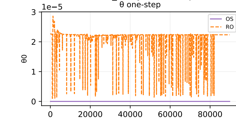
Oracle theta fit — ivtt_analytic — sample 680
