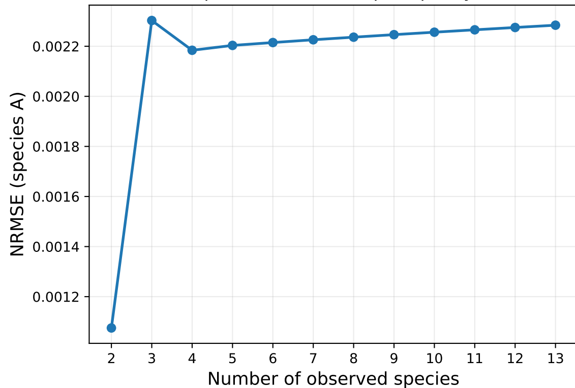
Species A — one-step fit quality
