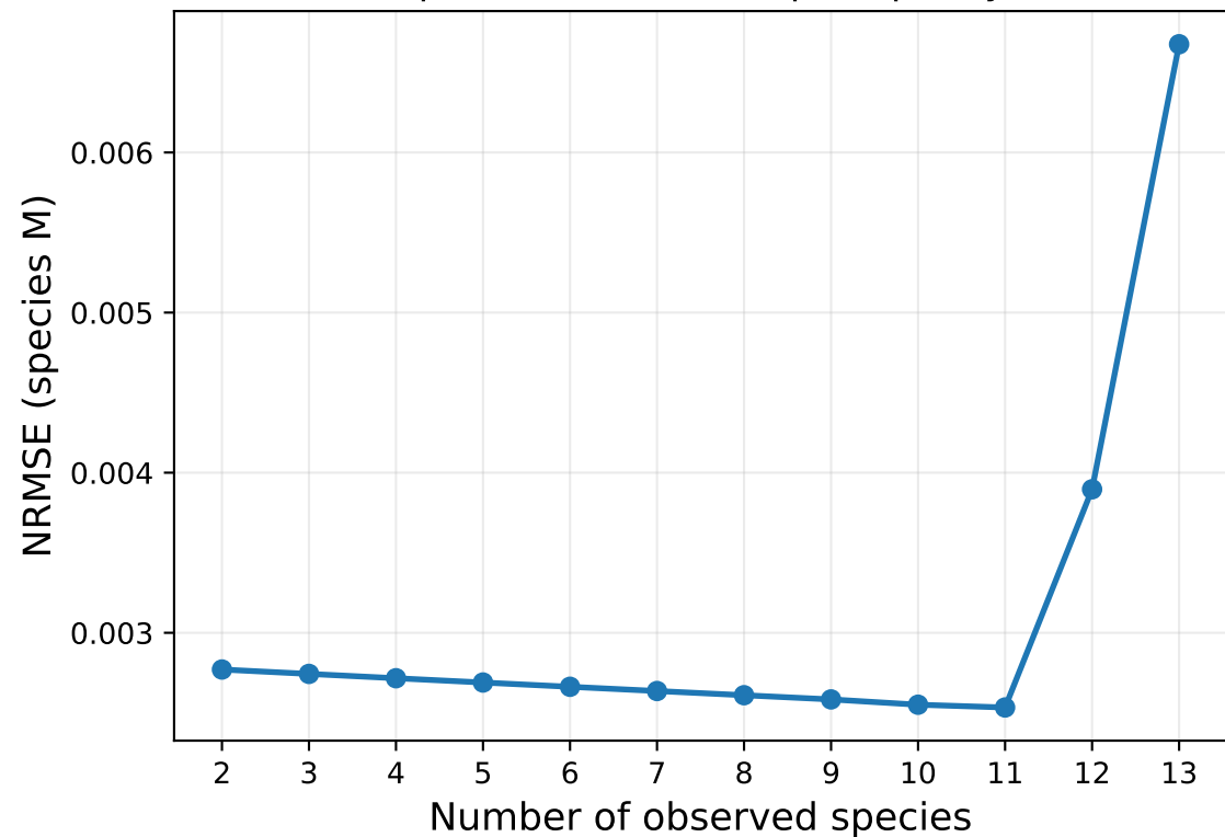
Species M — one-step fit quality
