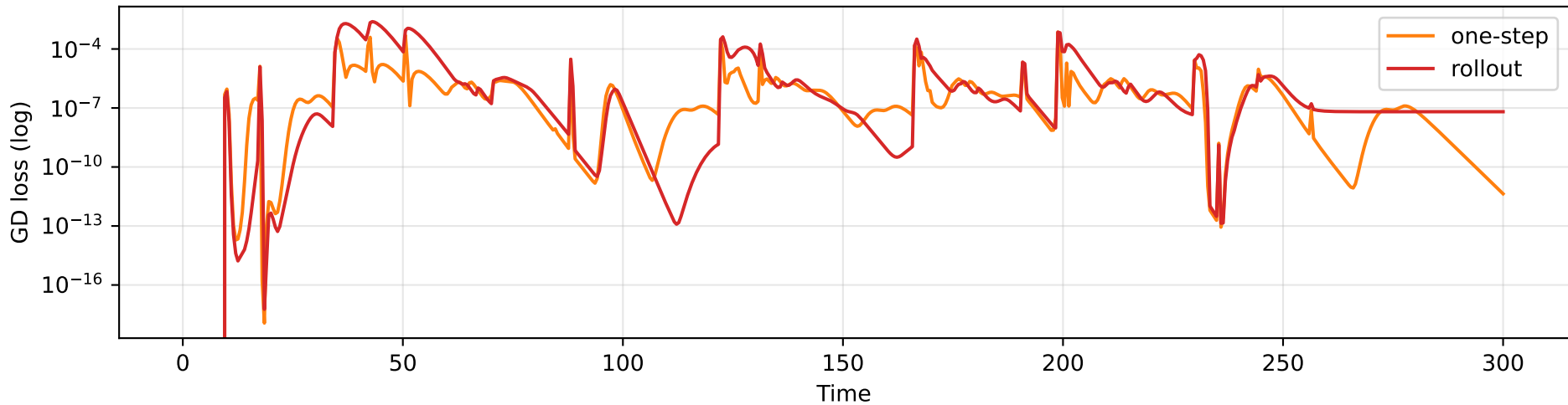
Per-step GD loss at convergence — reduced12_with_M
