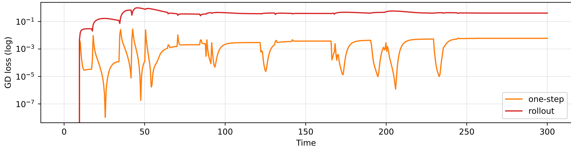
Per-step GD loss at convergence — reduced2
