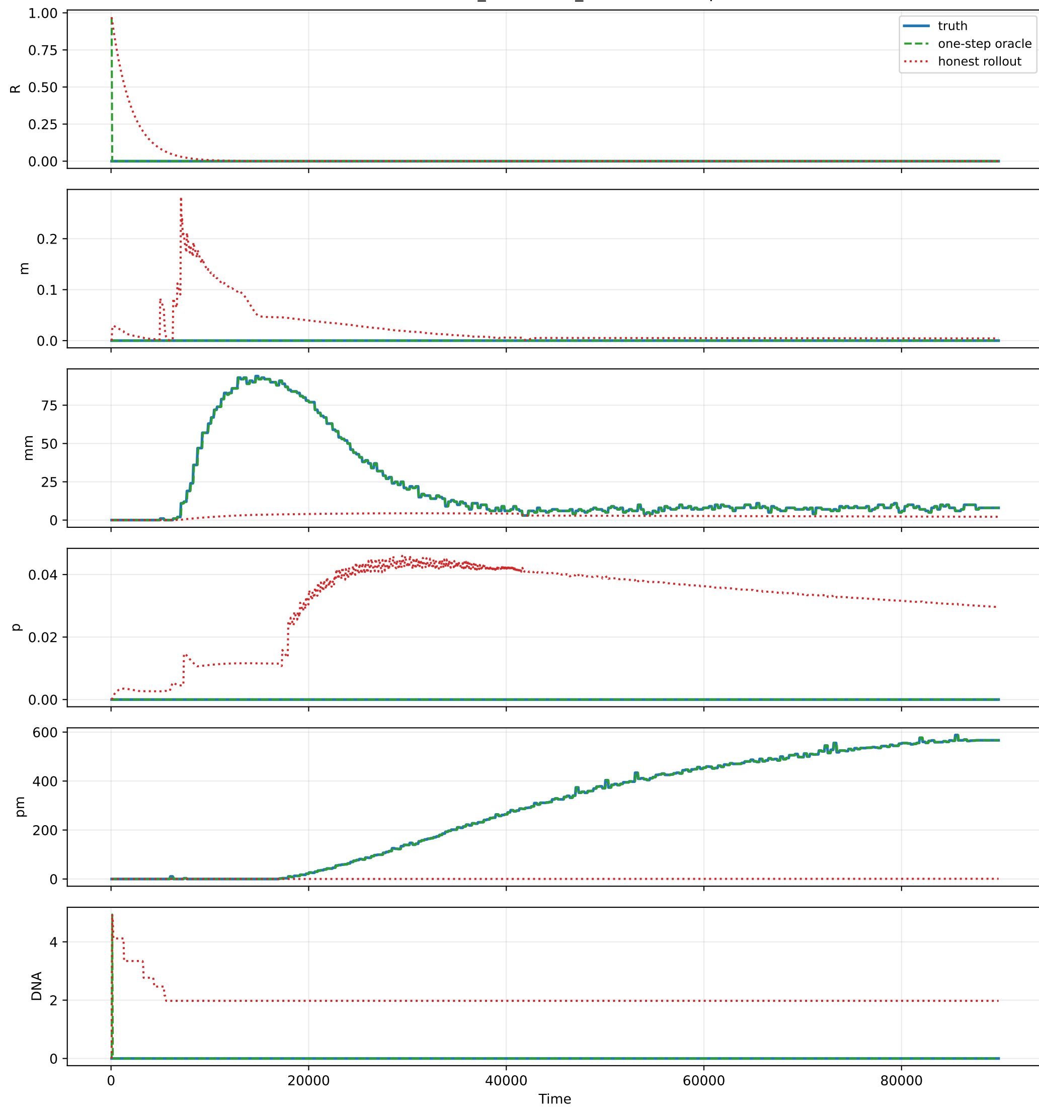
Oracle theta fit — txtl_maturation_dna (P=6) sample 0
