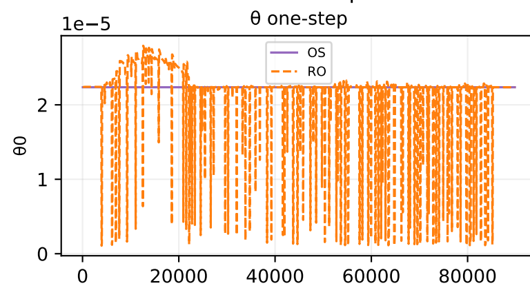
Oracle theta fit — sample 40
