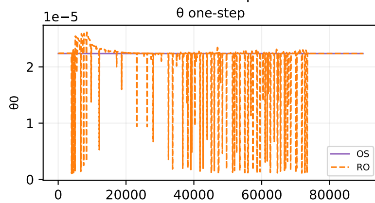
Oracle theta fit — sample 56
