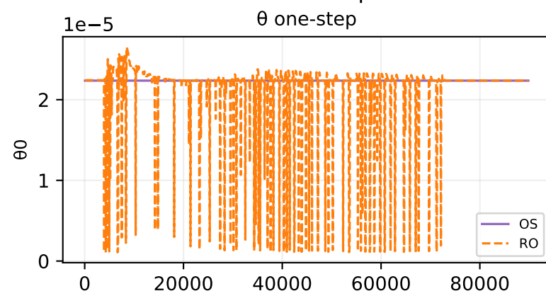
Oracle theta fit — sample 57
