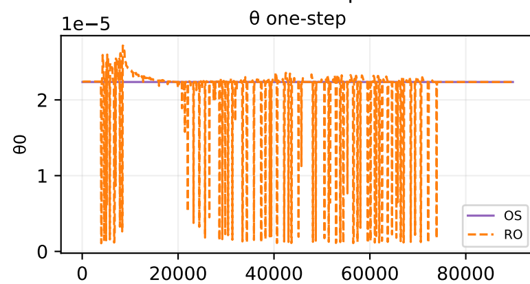
Oracle theta fit — sample 58
