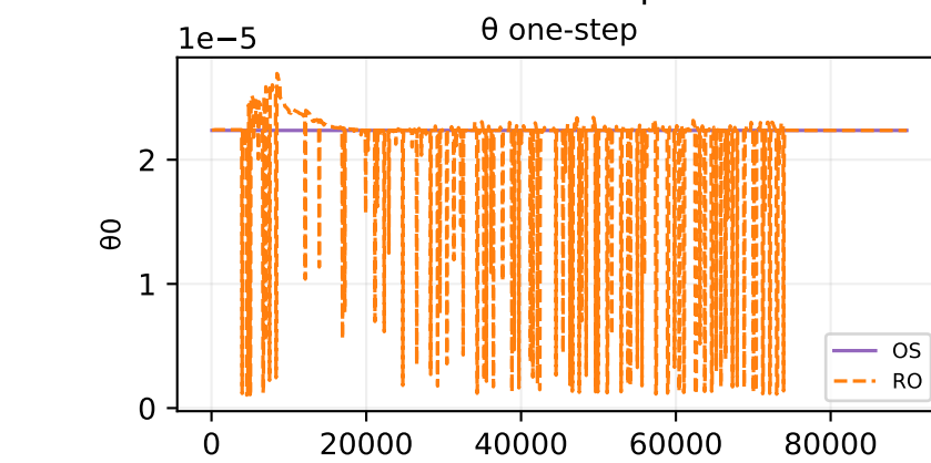
Oracle theta fit — sample 60
