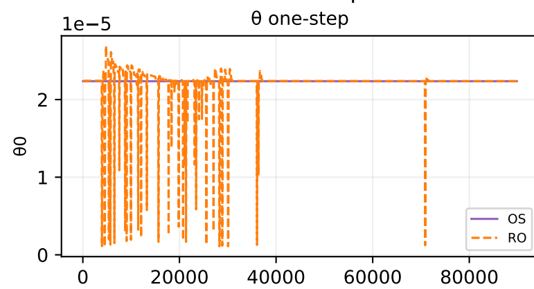
Oracle theta fit — sample 87
