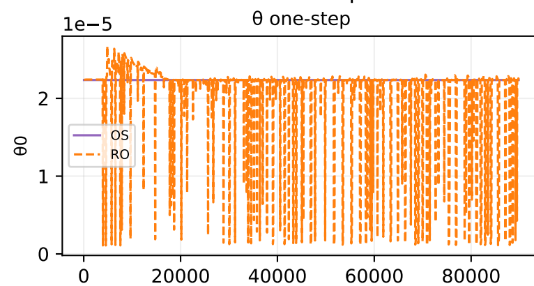
Oracle theta fit — sample 90
