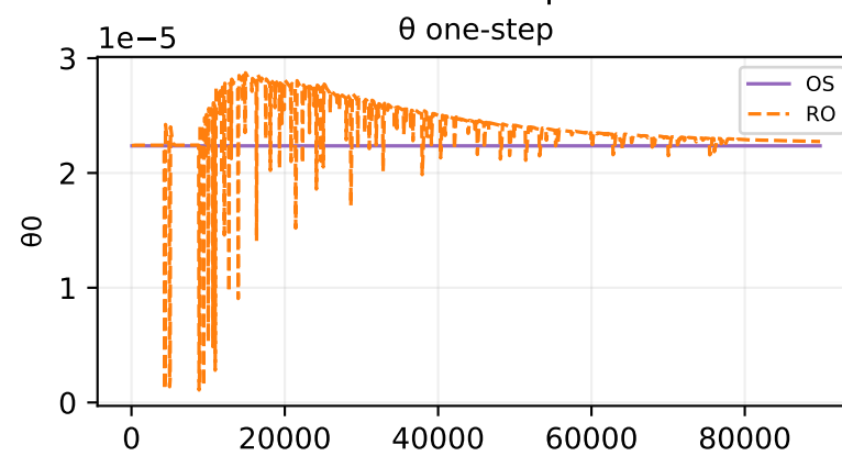
Oracle theta fit — sample 112
