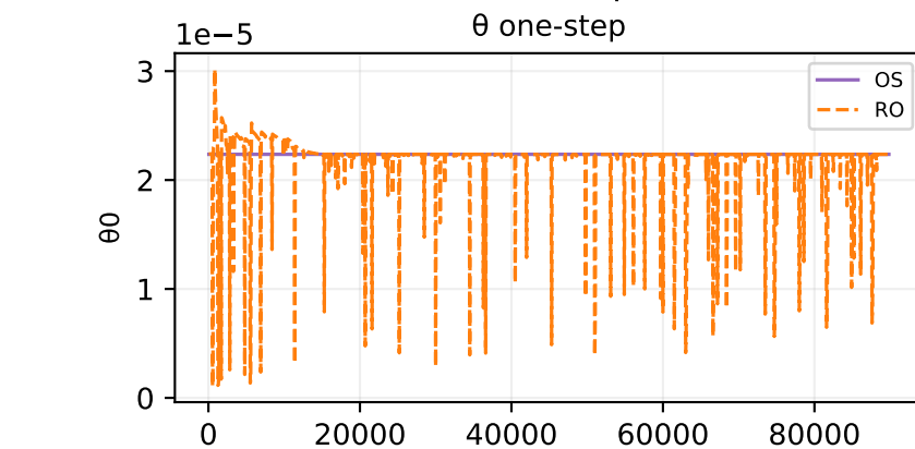
Oracle theta fit — sample 123
