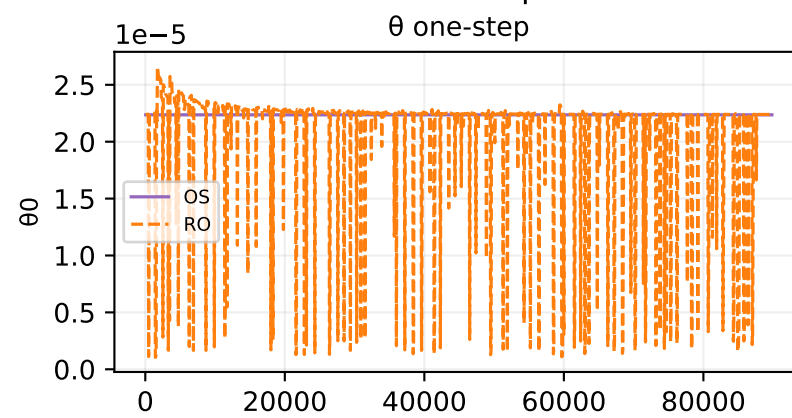
Oracle theta fit — sample 132
