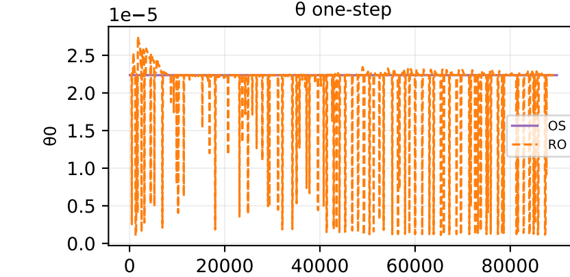
Oracle theta fit — sample 134
