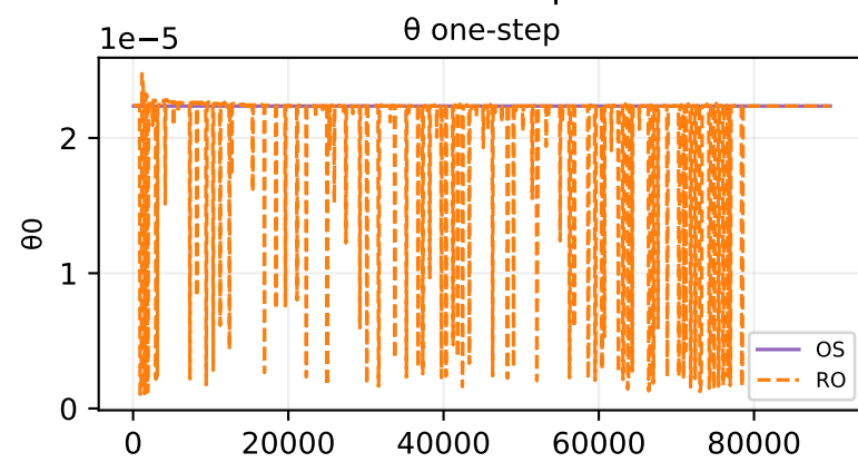
Oracle theta fit — sample 145
