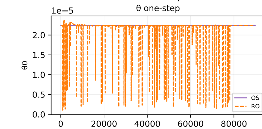
Oracle theta fit — sample 165
