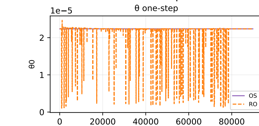
Oracle theta fit — sample 167
