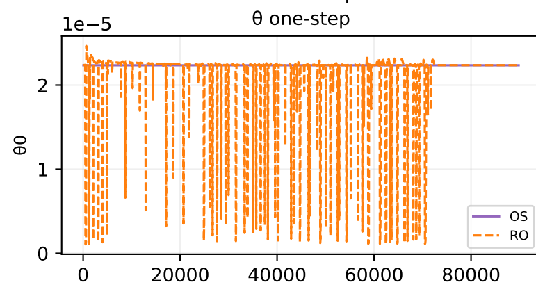
Oracle theta fit — sample 178
