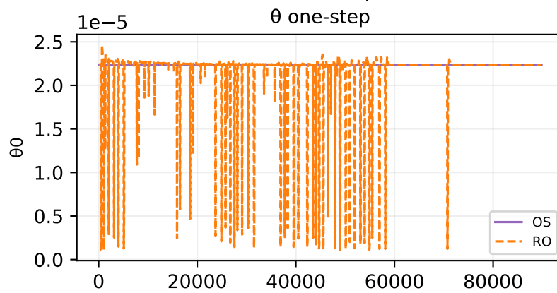
Oracle theta fit — sample 179
