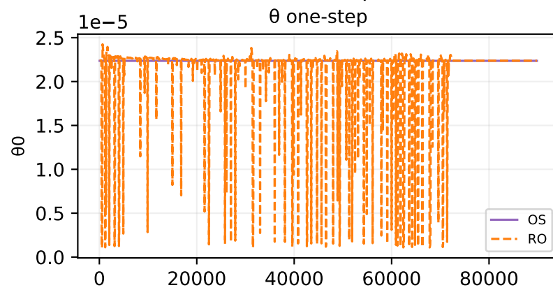
Oracle theta fit — sample 184
