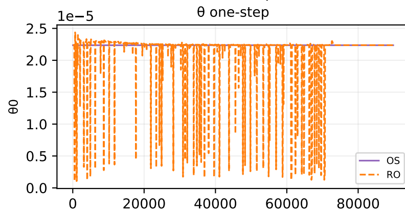
Oracle theta fit — sample 186
