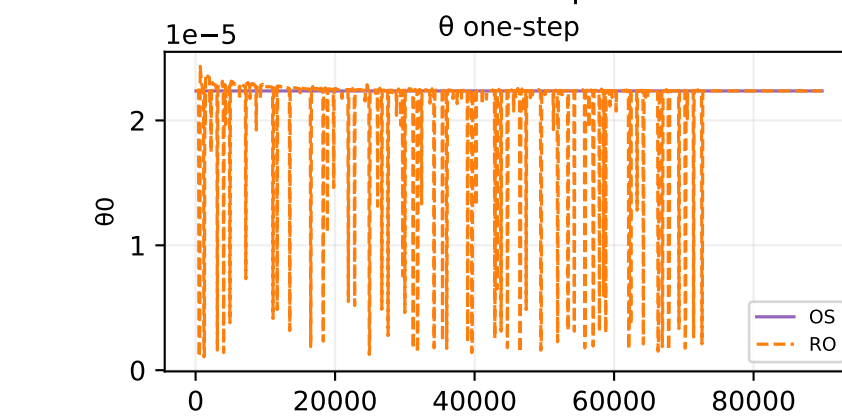
Oracle theta fit — sample 191
