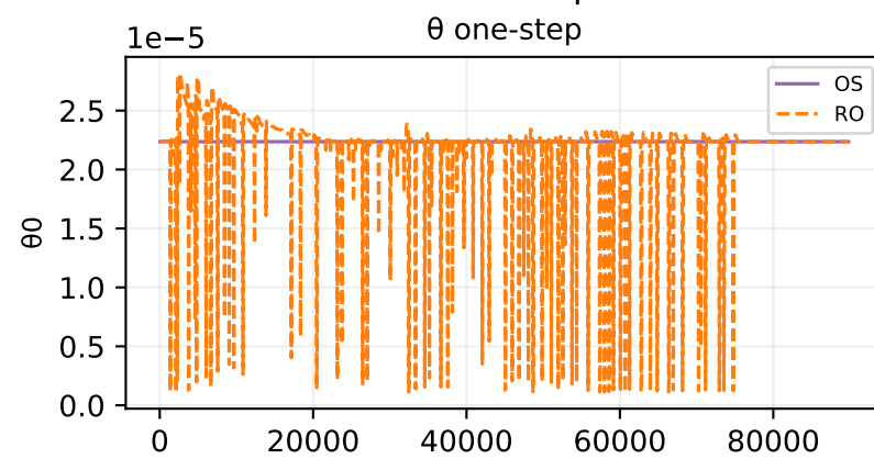
Oracle theta fit — sample 192
