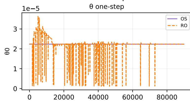
Oracle theta fit — sample 203
