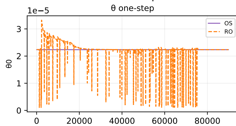
Oracle theta fit — sample 214
