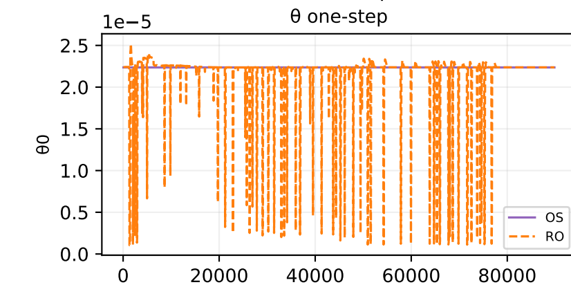
Oracle theta fit — sample 280
