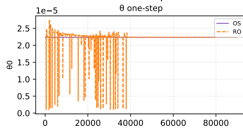
Oracle theta fit — sample 295
