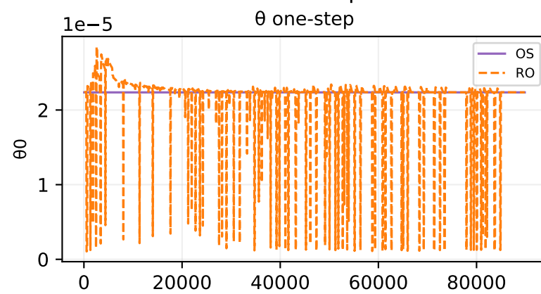
Oracle theta fit — sample 298
