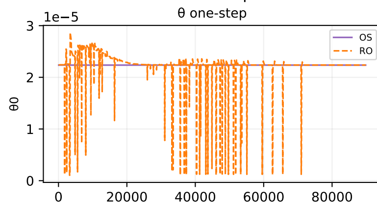
Oracle theta fit — sample 309
