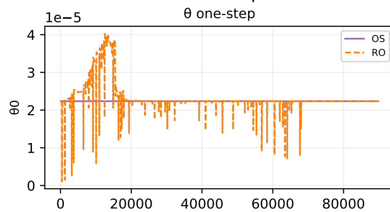
Oracle theta fit — sample 359
